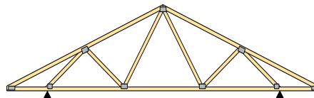
DOUBLE CANTILEVER
